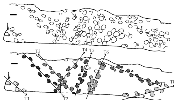
Fig. 2. Map of the Coisia site (top) and interpretative map without isolated footprints (bottom); Scale bar: 1 m.
