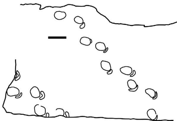
Fig. 3. Enlargement of trackways 1 and 2. Scale bar: 1 m.
